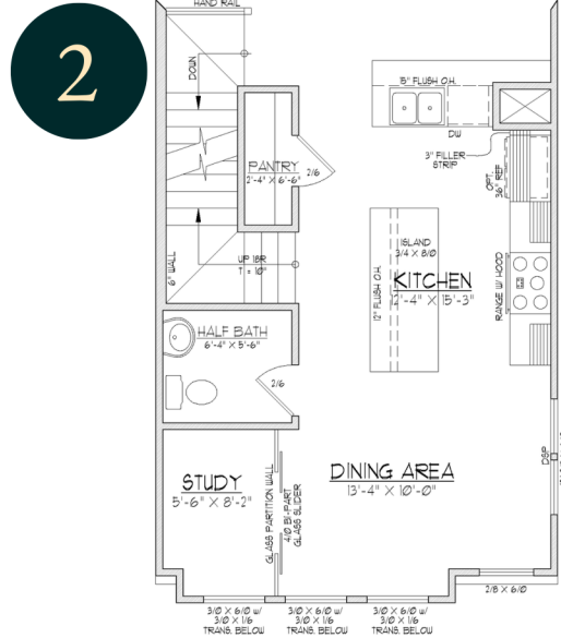
SECOND FLOOR PLAN B w/ OPT. STUDY
