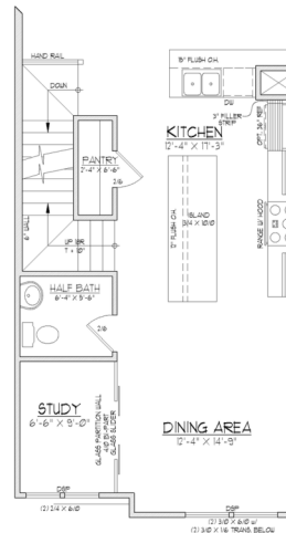
SECOND FLOOR PLAN A w/ OPT. STUDY
