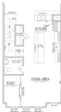
SECOND FLOOR PLAN B w/ OPT. STUDY
