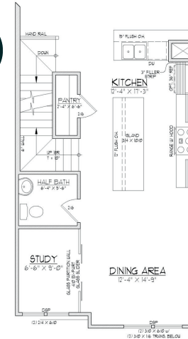
SECOND FLOOR PLAN A w/ OPT. STUDY
