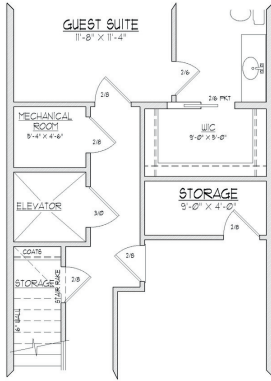
FIRST FLOOR PLAN w/ OPT. ELEVATOR
