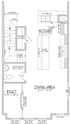
SECOND FLOOR PLAN B w/ OPT. STUDY
