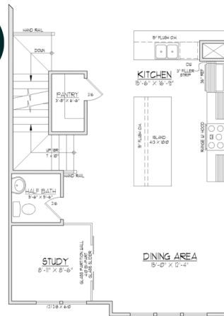
SECOND FLOOR PLAN A w/ OPT. STUDY
