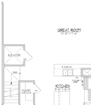
SECOND FLOOR PLAN w/ OPT. ELEVATOR
